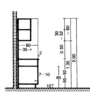
17 Section through kitchen units: preferred measurements
